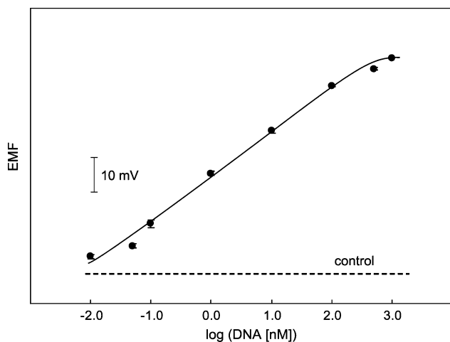
Figure 2. Calibration plot for the potentiometric monitoring of DNA with a sandwich array based on CdS quantum dot tags in 200- \mu\text{L} microwells (error bars: SD, N = 3 ). The dashed line corresponds to control signal (no target). Other conditions as in Figure 1.
