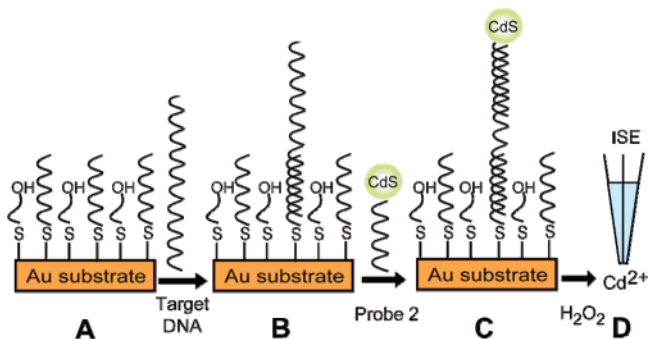
Scheme 1. Steps Involved in the Nanoparticle-Based Potentiometric Detection of DNA Hybridization a
